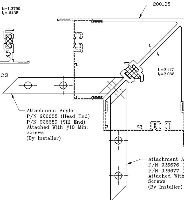
90° Corner Mullion
